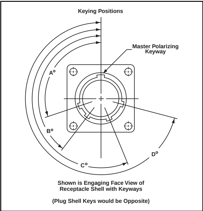
KEYING POSITIONS
