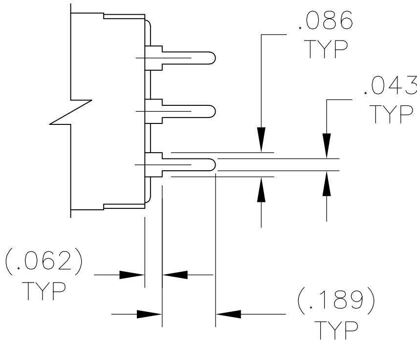
PC TERMINAL
