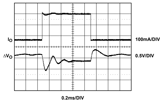
FIGURE 14. LOAD TRANSIENT RESPONSE, V_{IN} = 5V , V_O = 12V , I_O = 50mA TO 300mA
