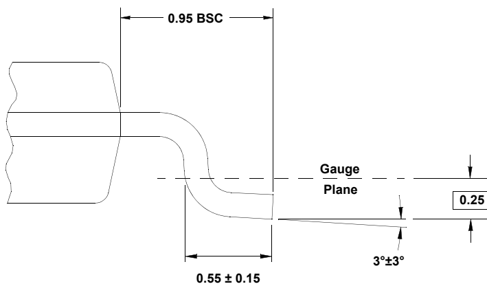
DETAIL "X"
