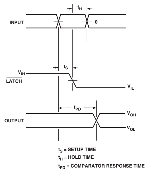
Figure 4. Latch Timing
