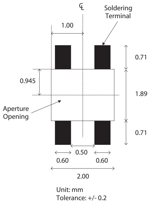
Figure A2. Recommended Land Pattern
