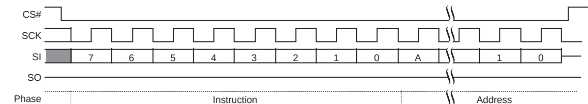
Figure 10.45 Parameter Sector Erase (P4E 20h or 4P4E 21h) Command Sequence
