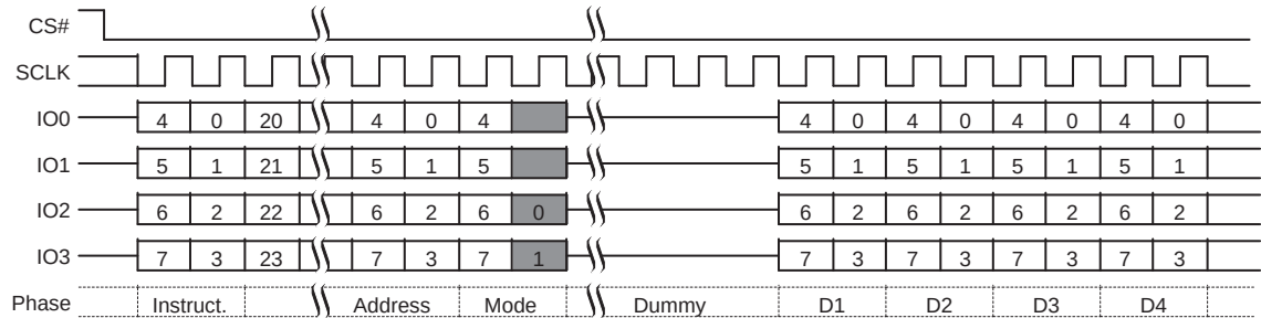
Figure 10.33 Quad I/O Read Command Sequence (3-Byte Address, EBh [CR2V[7]=0]) QPI Mode
