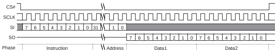
Figure 4.6 Single Bit Wide I/O Command without Latency
