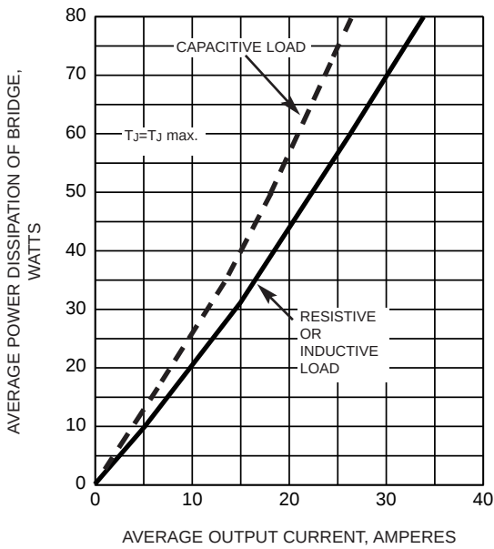
FIG. 3 - MAXIMUM POWER DISSIPATION
