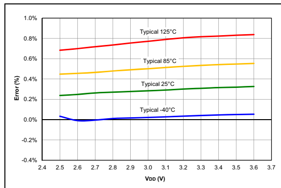
FIGURE 36-94: FVR Voltage Error (2x), PIC16LF18313/18323 Only
