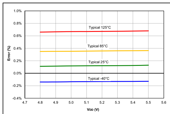
FIGURE 36-96: FVR Voltage Error (4x), PIC16F18313/18323 Only
