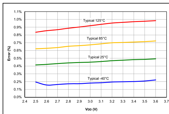
FIGURE 36-92: Typical FVR Voltage (1x), PIC16LF18313/18323 Only
