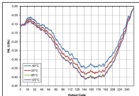
FIGURE 36-72: Typical DAC INL Error, VDD = 5.0V, VREF = External 5V, PIC16F18313/18323 Only
