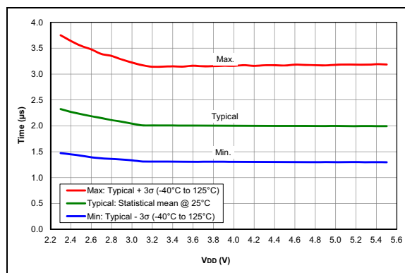
FIGURE 36-68: ADC RC Oscillator period, PIC16F18313/18323 Only
