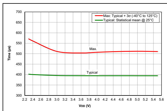
FIGURE 36-113: Wake From Sleep, VREGPM = 1, LFINTOSC, PIC16F18313/18323 Only
