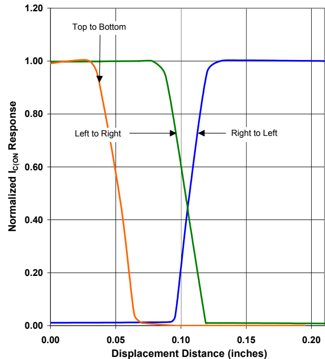
OPB610 - Flag Next to Sensor
