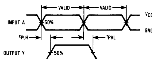
Figure 2. Switching Waveforms
