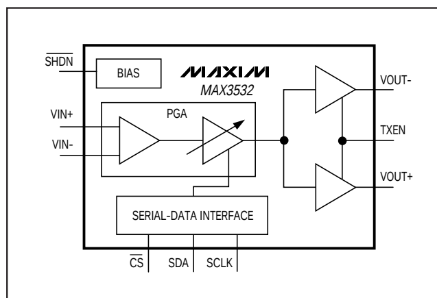
Figure 1. Functional Diagram
