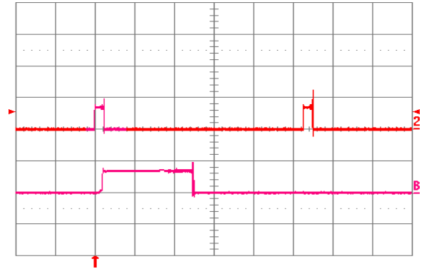
Fig. 6.0V.18: Load current (top trace, 20 A/div., 20 ms/div.) into a 10 mΩ short circuit during restart, at V_{in} = 24V . Bottom trace (20 A/div., 2 ms/div.) is an expansion of the on-time portion of the top trace.
