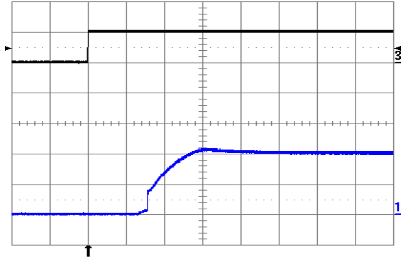
Fig. 1.0V.10: Turn-on transient at full rated load current (resistive) plus 10,000 \mu F at V_{in} = 24V , triggered via ON/OFF pin. Top trace: ON/OFF signal (5 V/div.). Bottom trace: output voltage (0.5 V/div.). Time scale: 1 ms/div.
