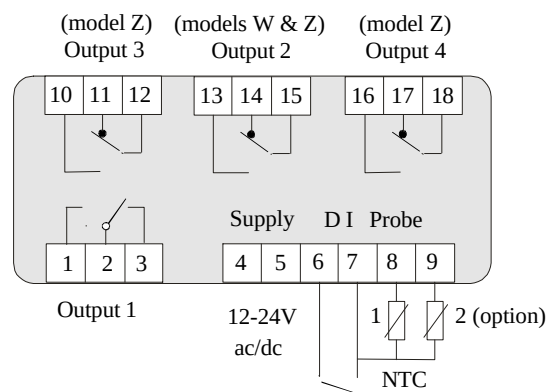
IR32 Models NTC only
