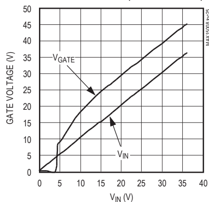
PROTECTOR GATE VOLTAGE vs. INPUT VOLTAGE (MAX15008 ONLY)
