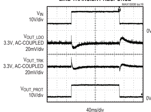
LINE-TRANSIENT RESPONSE
