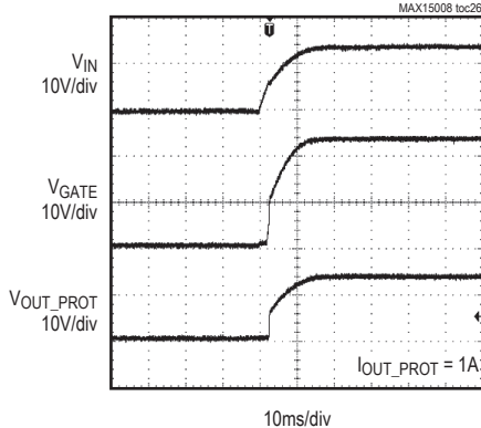
PROTECTOR STARTUP RESPONSE (MAX15008 ONLY)
