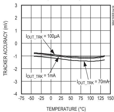
TRACKER ACCURACY ( V_{FB\_TRK} = V_{ADJ} ) vs. TEMPERATURE
