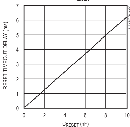
RESET TIMEOUT DELAY vs. C_RESET
