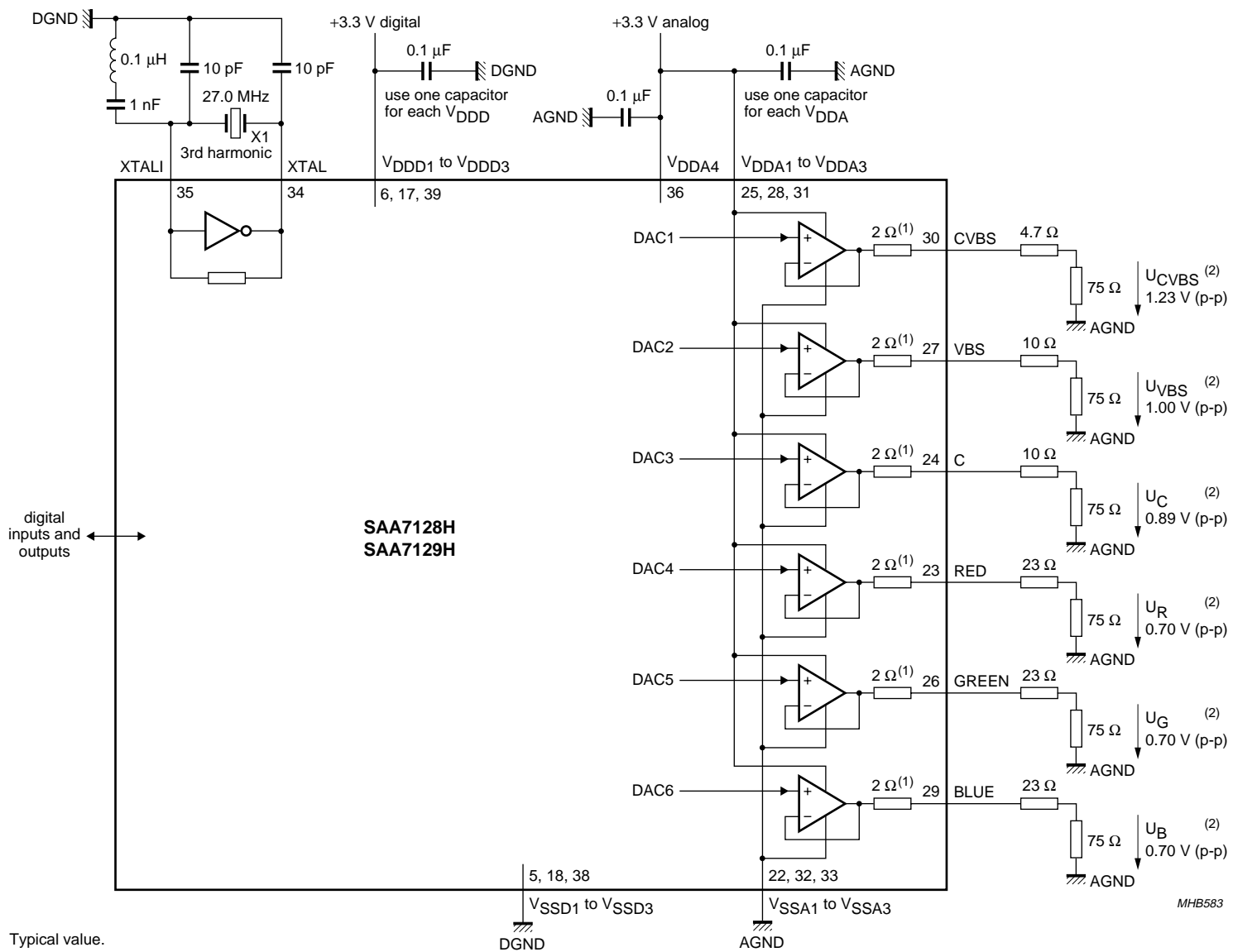
Fig.24 Application circuit.
