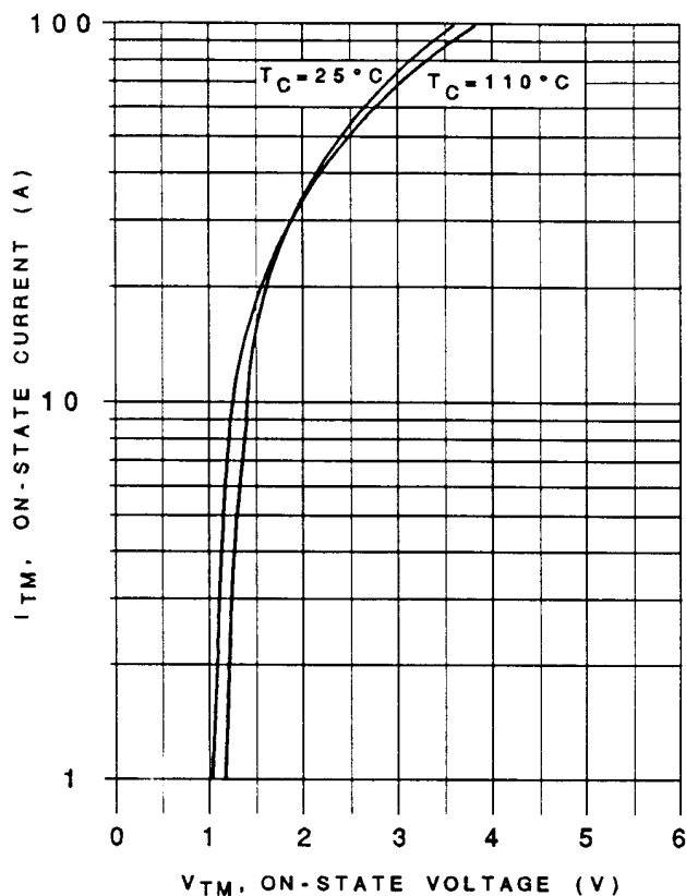
MAXIMUM ON-STATE CHARACTERISTICS
