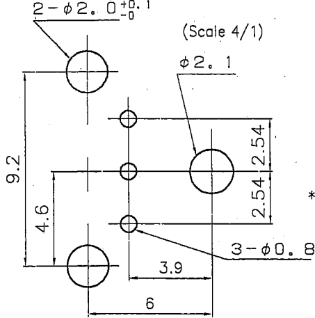
Example of mounting drawing from solder side Unspecified tolerance \pm 0.1
