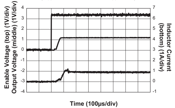
Soft Start
