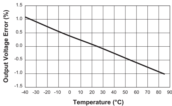
Output Voltage Error vs. Temperature ( V_{OUT} = 1.8V ; I_{OUT} = 1A )
