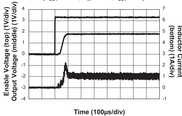
Soft Start
