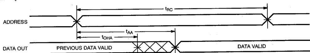
Read Cycle No. 1 [13, 14]
