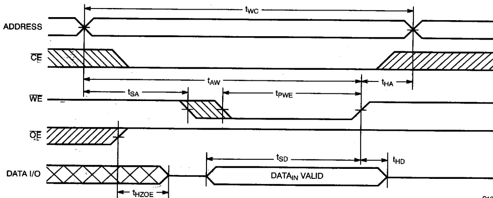
Write Cycle No. 1 (WE Controlled) [11, 16, 17]
