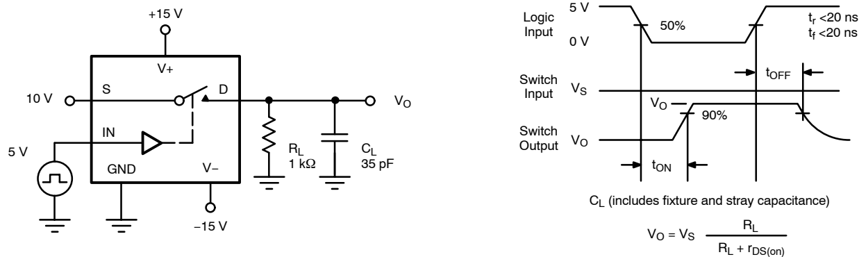
FIGURE 2. Switching Time
