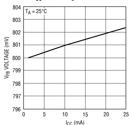
Reference Voltage vs V_{CC} Shunt Regulator Current
