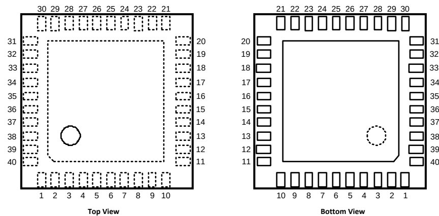
Figure 3. 40-Pin WQFN Package Number RSB0040A
