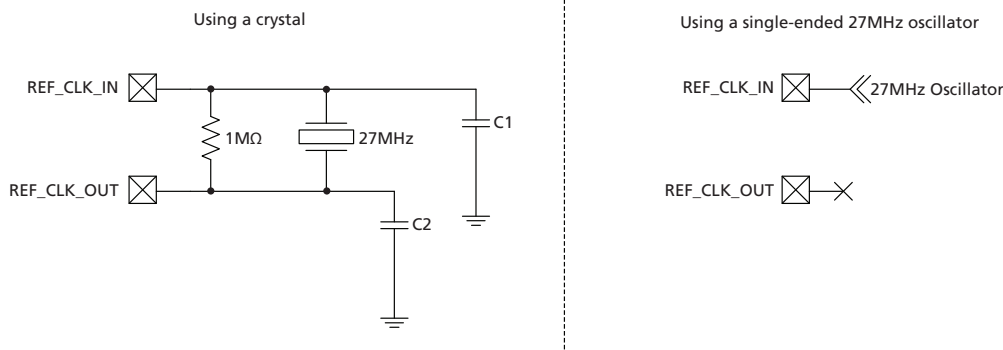
Figure 3-5: Crystal Oscillator
