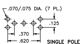
SINGLE POLE
