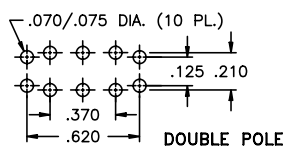
DOUBLE POLE
