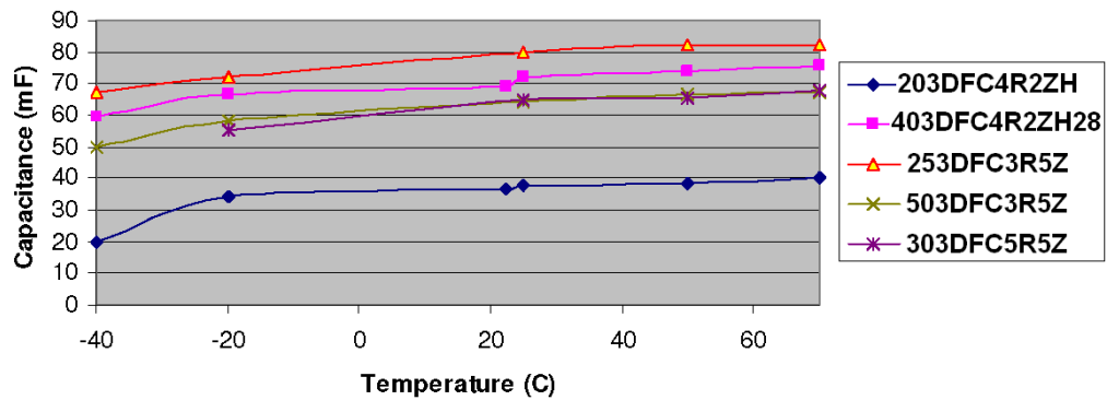
Capacitance vs. Temperature
