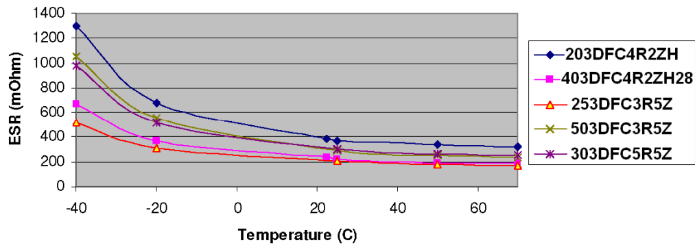
ESR vs. Temperature
