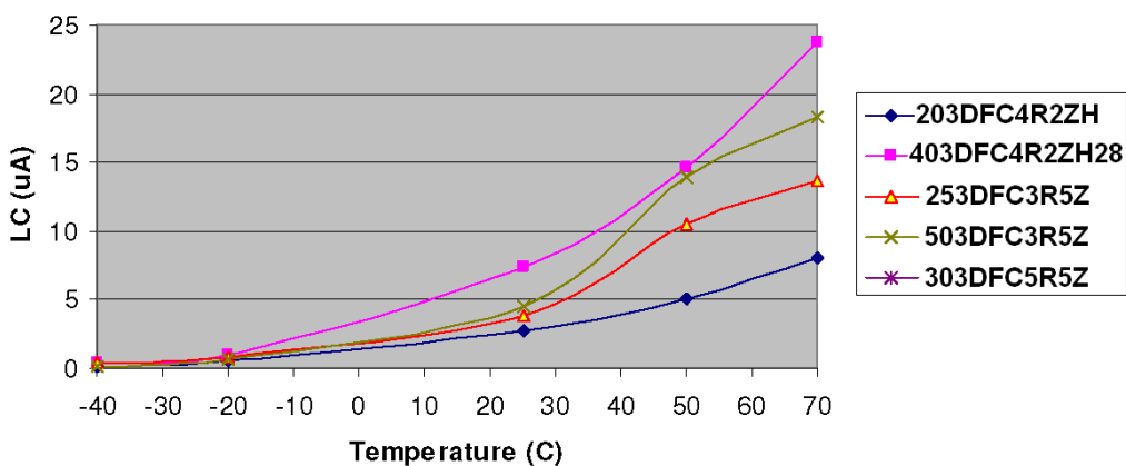
LC vs. temperature
