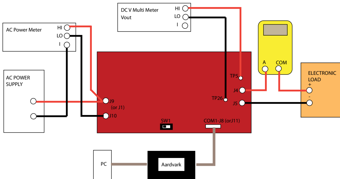
Figure 2 - Test configuration for the Evaluation Board
