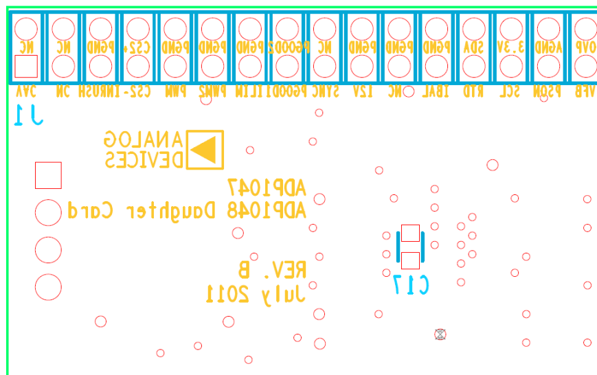
Figure 16 –Bottom Silkscreen
