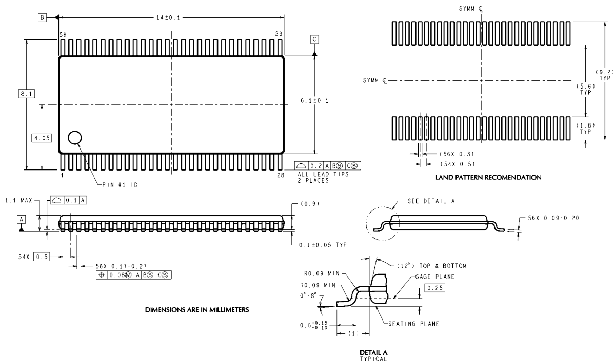
56-Lead Molded Thin Shrink Small Outline Package, JEDEC Dimensions shown in millimeters only Order Number DS90CR286AMTD, DS90CR286AQMT NS Package Number MTD56
