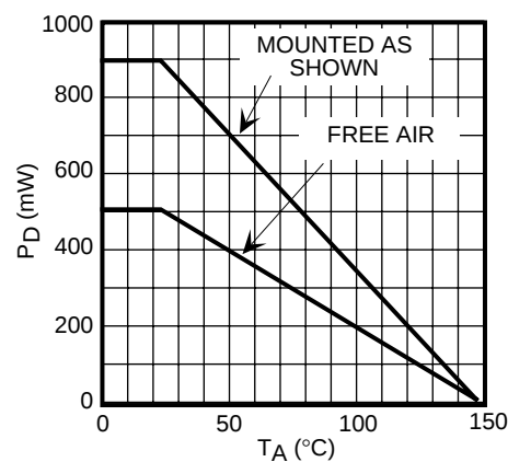
SOT-89 POWER DISSIPATION CURVE
