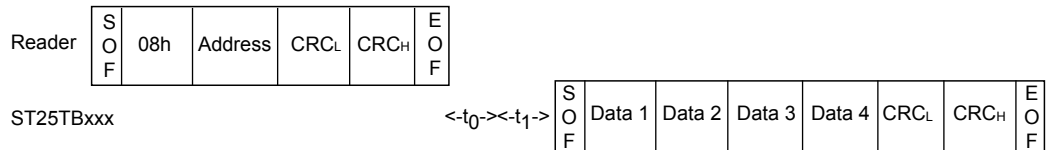
Figure 53. Read_block frame exchange between reader and ST25TB512-AC
