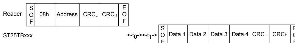
Figure 38. Read_block frame exchange between reader and ST25TB512-AC
