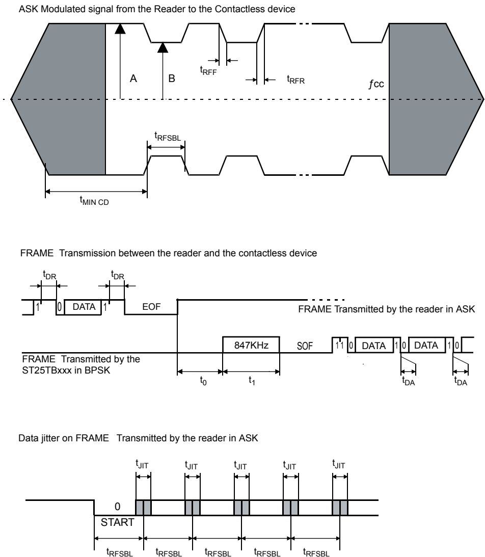
Figure 46. ST25TB512-AC synchronous timing, transmit and receive
