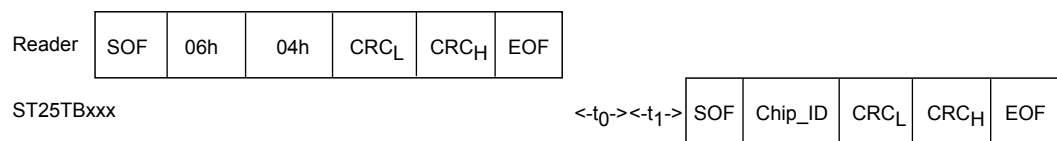
Figure 48. Pcall16 frame exchange between reader and ST25TB512-AC
