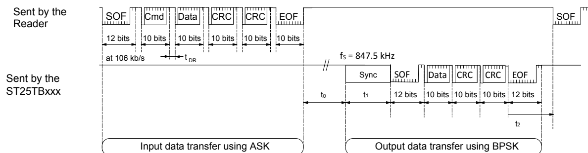
Figure 10. Example of a complete transmission frame
