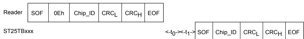
Figure 50. Select frame exchange between reader and ST25TB512-AC
