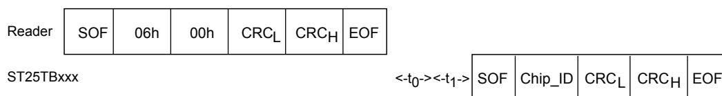
Figure 20. Initiate frame exchange between reader and ST25TB512-AC
