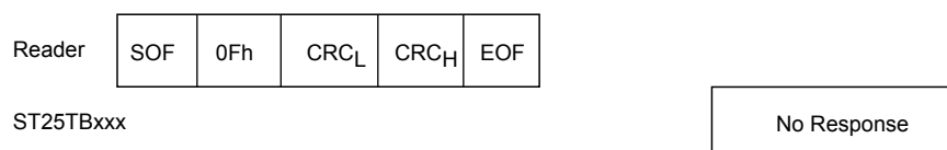
Figure 32. Completion frame exchange between reader and ST25TB512-AC
