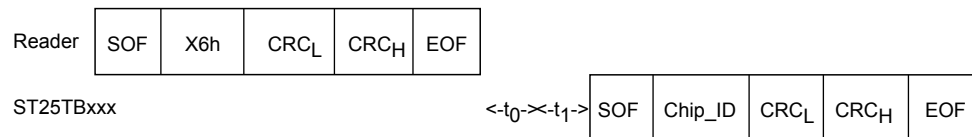
Figure 49. Slot_marker frame exchange between reader and ST25TB512-AC
