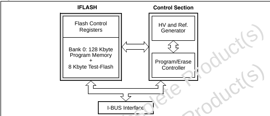
Figure 5. Flash structure
