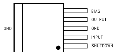
Figure 2. TO-263, Top View
