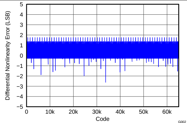
Figure 2. Differential Nonlinearity
