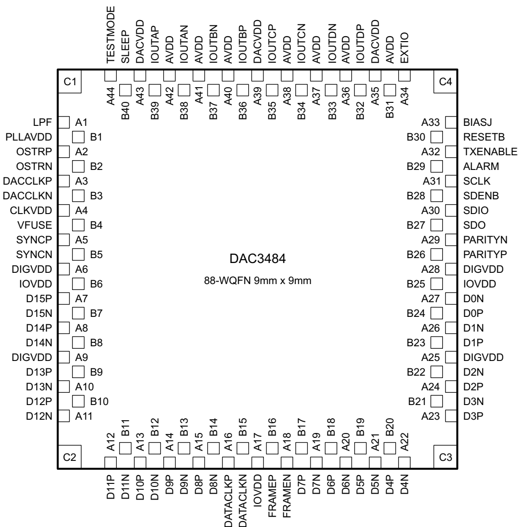
RKD Package 88-Pin WQFN Top View
