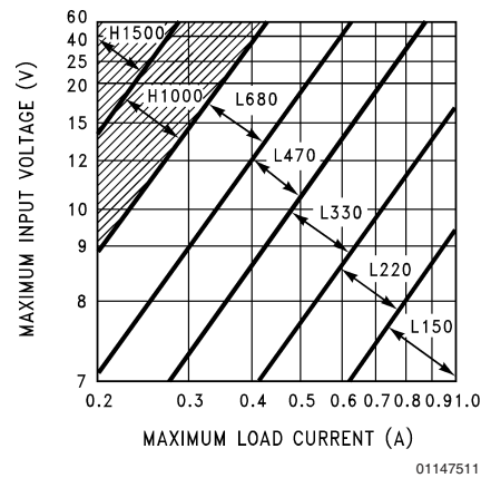
FIGURE 4. LM2575(HV)-5.0
