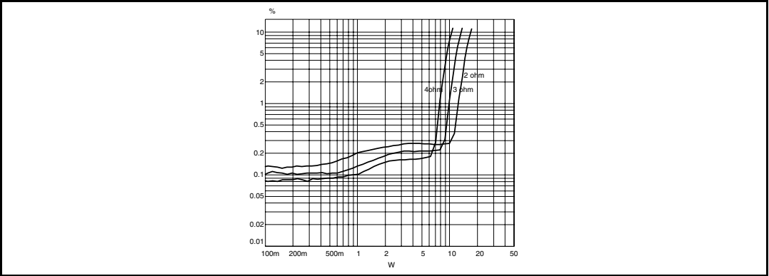
Figure 36. THD+N vs. output power, single ended, 1 kHz, half-bridge binary
