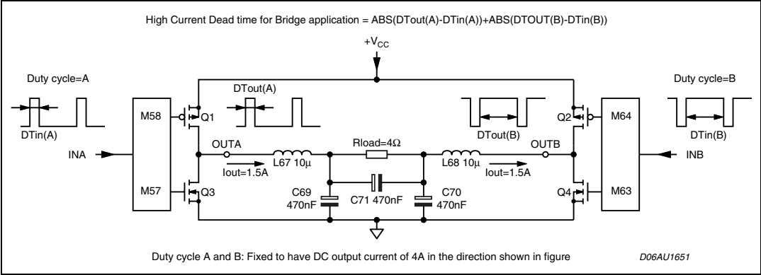
Figure 12. Test circuit 2
