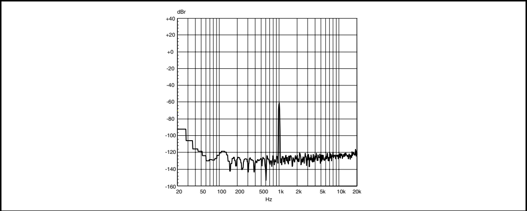
Figure 30. FFT -60 dBFS 1 kHz, 8 \Omega
