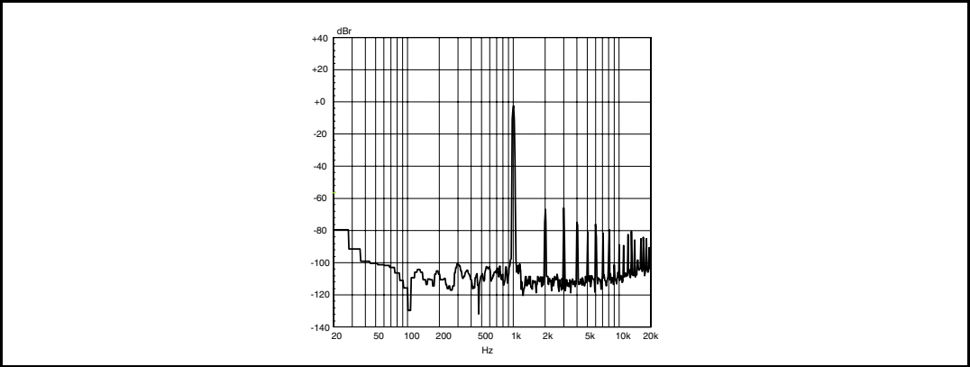
Figure 27. FFT 0 dBFS 1 kHz, 8 \Omega
