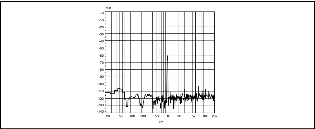
Figure 43. FFT -60 dB, single ended, 1 kHz, 4 \Omega
