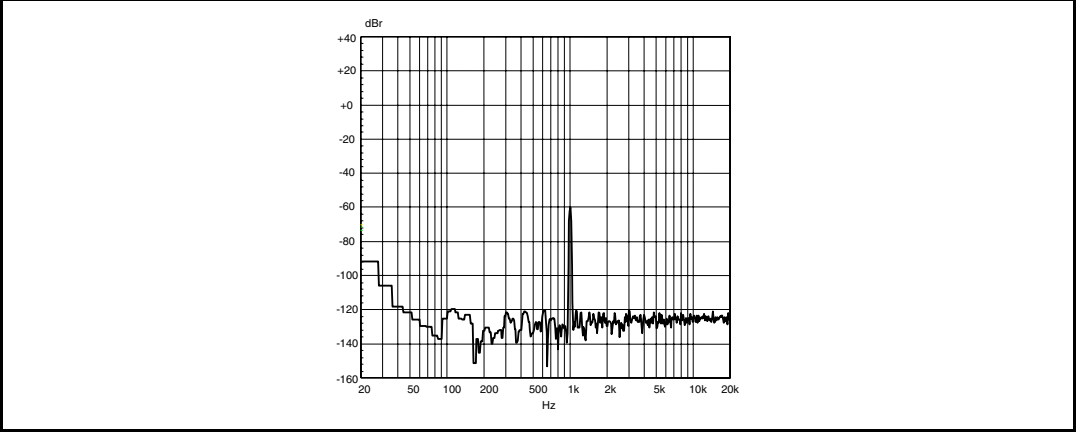
Figure 32. FFT -60 dBFS 1 kHz, 4 \Omega
