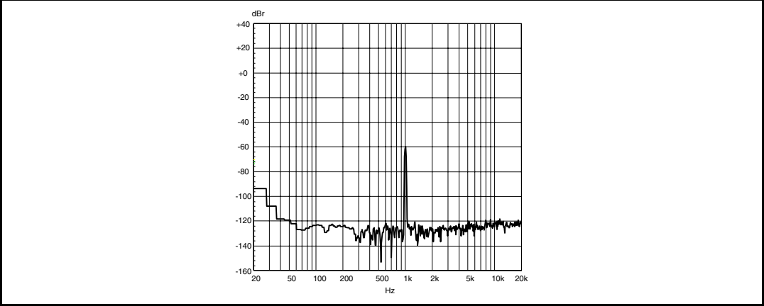
Figure 31. FFT -60 dBFS 1 kHz, 6 \Omega
