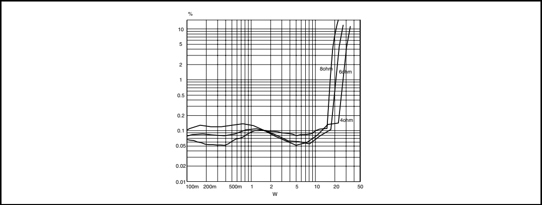
Figure 24. THD vs. output power, BTL, 1 kHz
