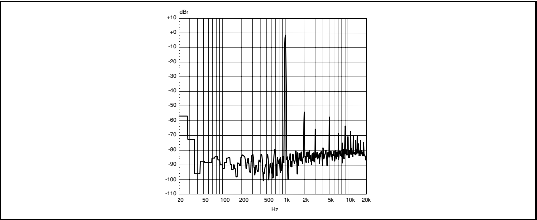
Figure 42. FFT -60 dB, single ended, 1 kHz, 2 \Omega
