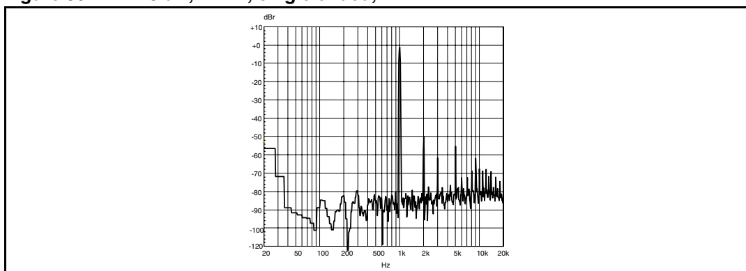
Figure 40. FFT 0 dB, 1 kHz, single ended, 3 \Omega
