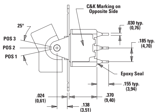
Part number shown: 7101J12QE2
