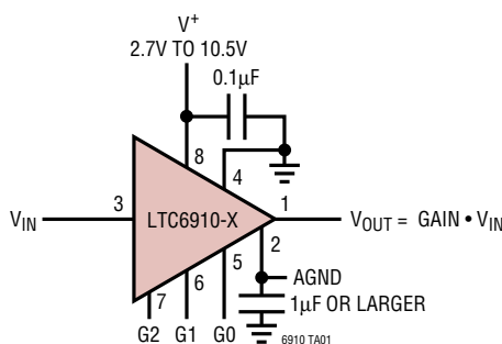
Single Supply Programmable Amplifier
