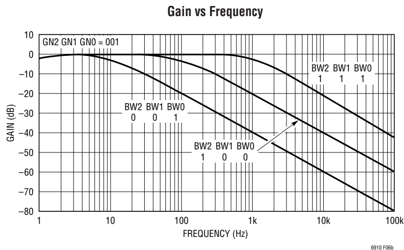
Figure 8. Low Noise AC Amplifier with Programmable Gain and Bandwidth
