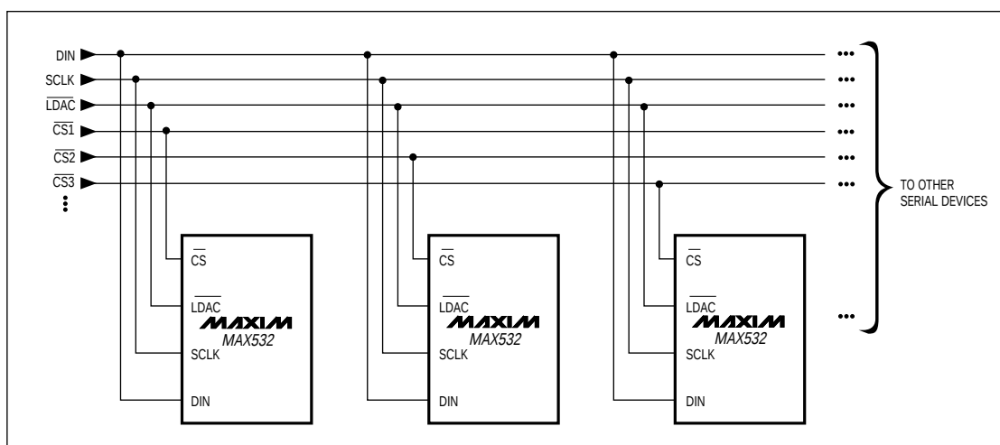
Figure 7. Multiple devices sharing a common DIN line may be simultaneously updated by bringing LDAC low. CS1, CS2, CS3, ... are driven separately, thus controlling which data are written to devices 1, 2, 3, ...
