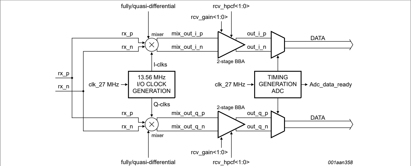
Figure 21. Block diagram of receiver circuitry
