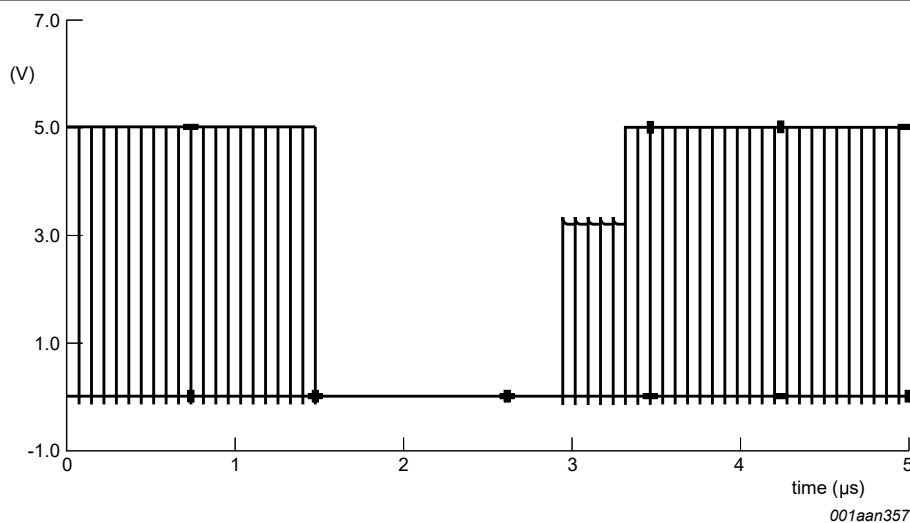
Figure 20. Example 2: overshoot_t1 = 0d; overshoot_t2 = 5d
