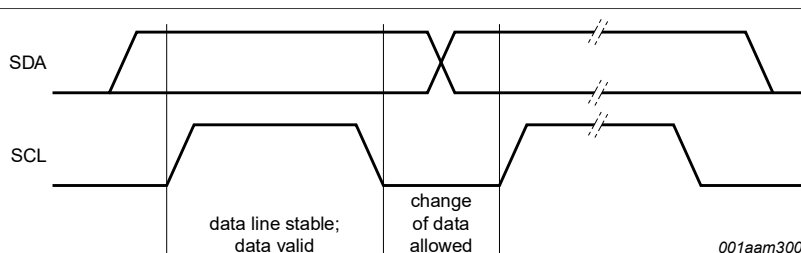
Figure 11. Bit transfer on the I 2 C-bus.
