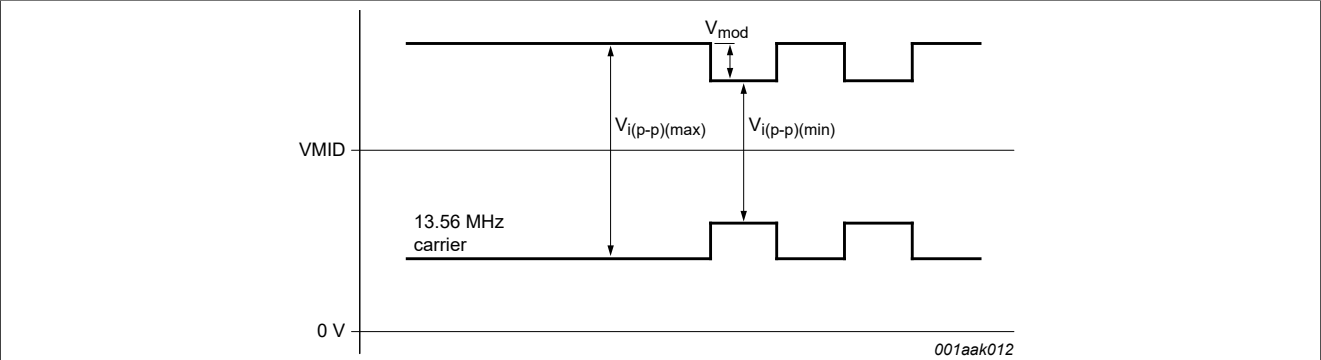
Figure 27. Pin RX input voltage
