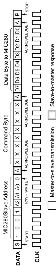
Figure 1. WRITE_BYTE Protocol
