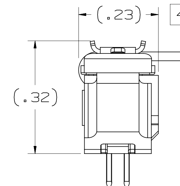
VERTICAL ASSEMBLY
