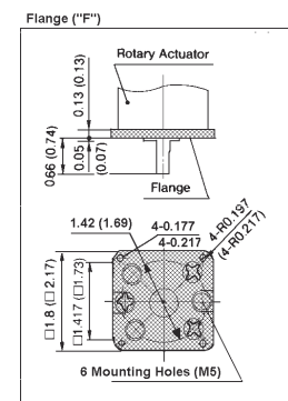
Dim for NCR1W20 ( ): Dim for NCRB1W30
