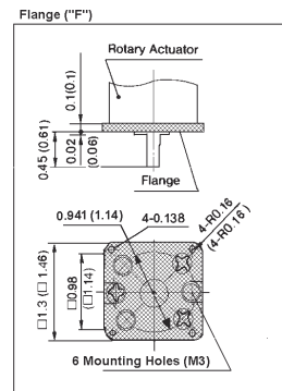
Dim for NCR1W10 ( ): Dim for NCRB1W15
