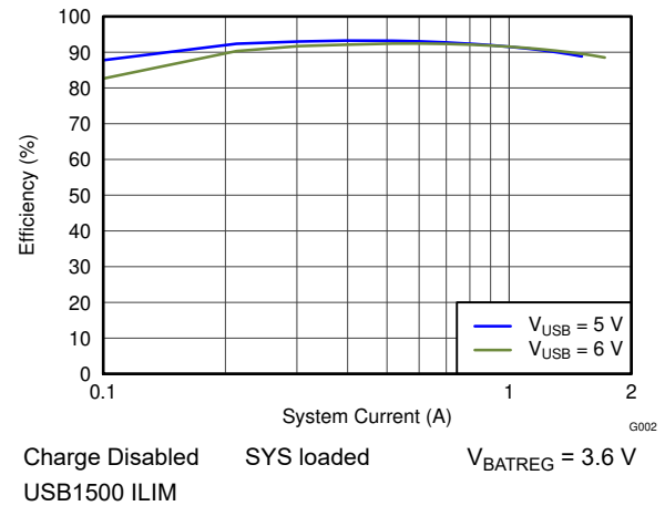
Figure 7-2. USB Efficiency
