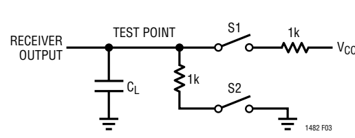
Figure 3. Receiver Timing Test Load
