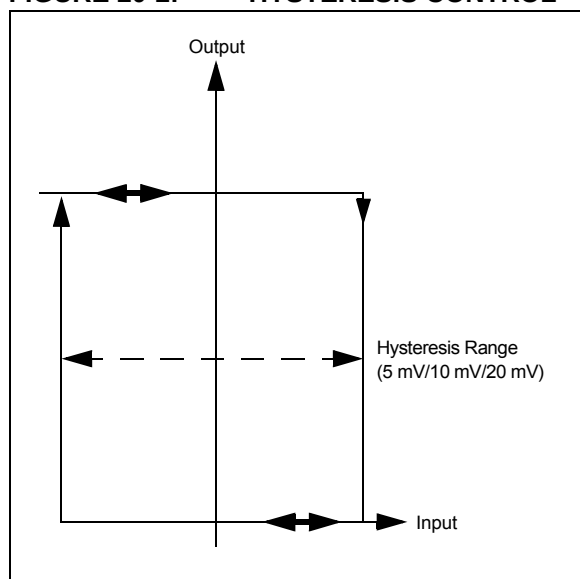
FIGURE 20-2: HYSTERESIS CONTROL
