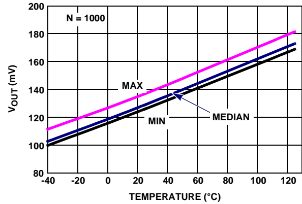
FIGURE 32. EL8173 V_{OUT} LOW vs TEMPERATURE, R_L = 1k , V_+ = 5V , V_- = 0V , V_{CM} = +2.5V
