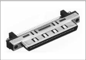
Straddle SMT type female connector for PCB HDRA-E68FT2-OM06+
