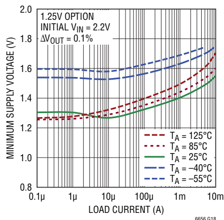
Minimum Supply Voltage vs Load Current
