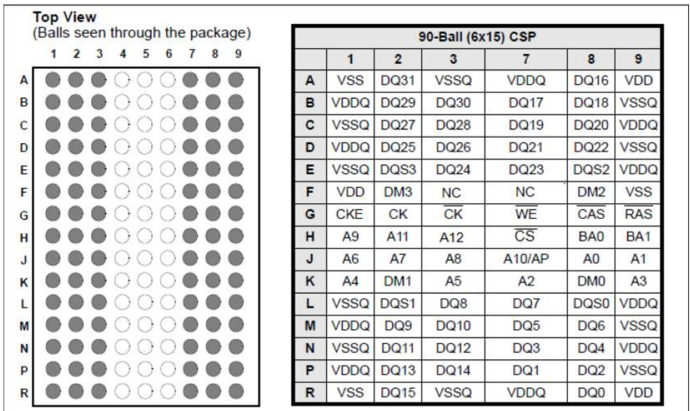
Figure 1 — PIN DESCRIPTION
