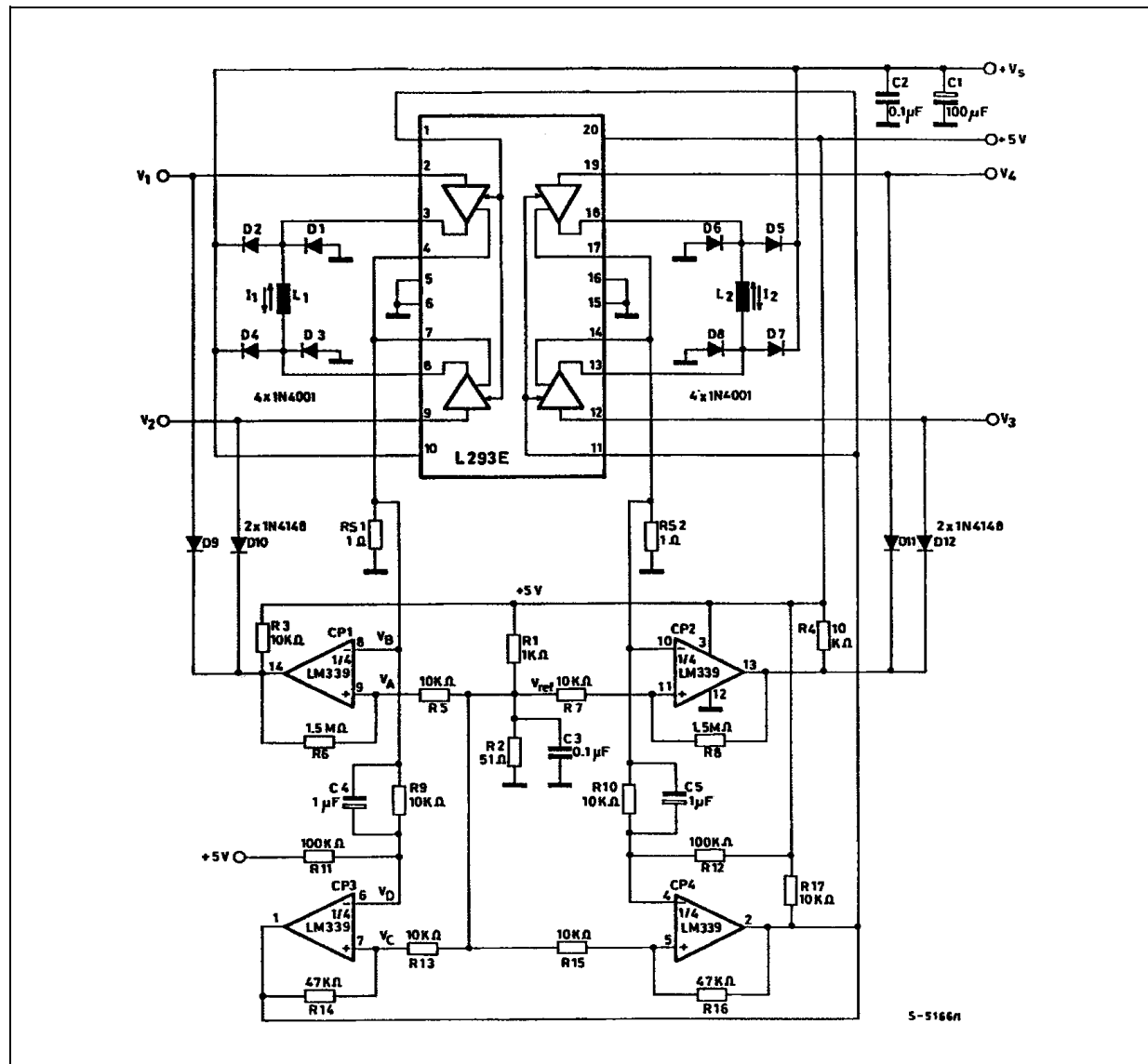
Figure 11. Stepping Motor Driver with Phase Current Control and Short Circuit Protection
