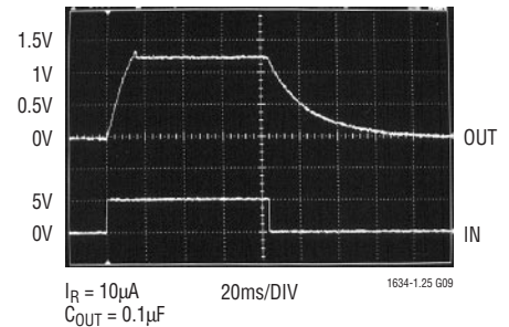
Response Time
