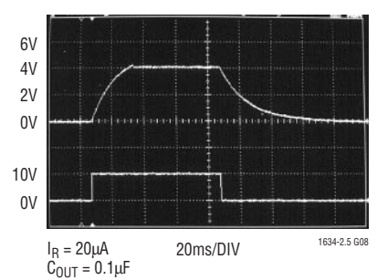
Response Time
